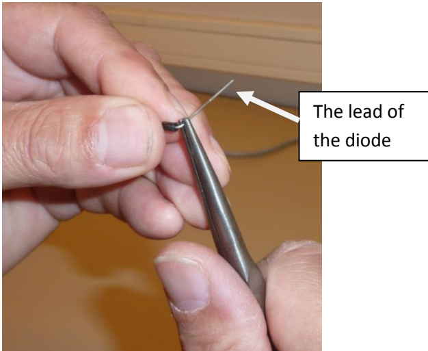
Fold and shorten the lead of the diode with the long nose pliers
