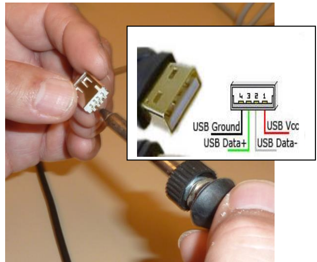
Solder the USB plug
